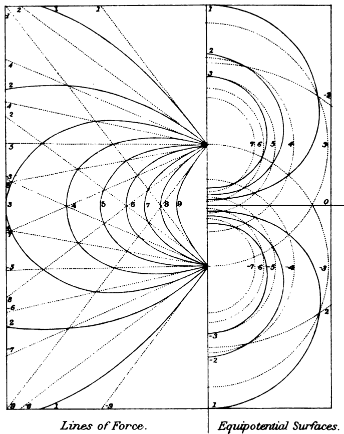
Method of drawing Lines of Force and Equipotential Surfaces.
