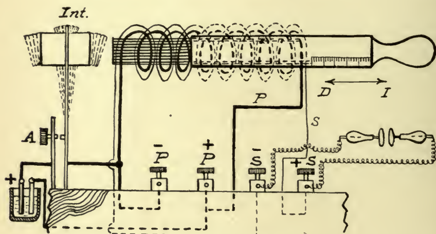
FIG. 28.—Medical induction coil.
