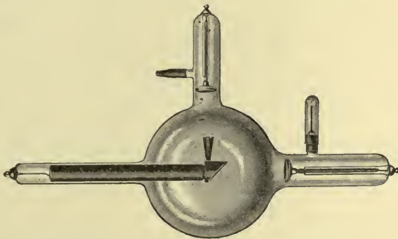
FIG. 212.—THE BI-CATHODE TUBE OF KOCH OF DRESDEN.—Koch asserts that where much inverse current must be overcome, this tube acts both as an X-ray and a ventril tube. He believes that, the anode being of a heavy design, a large quantity of current may be employed with a shortened exposure. (Kny-Scheerer Co.)
