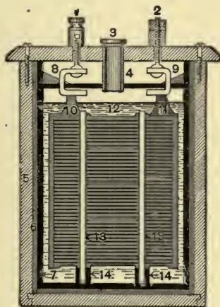
FIG. 5.—Diagrammatic view of the inner construction of a storage cell. (American Battery Company.) 1, positive binding post; 2, negative binding post; 3 rubber cap; 4, hard-rubber vent-tube; 5, oak case; 6, compound between rubber jar and oak case; 7, hard-rubber jar; 8, leaden lug attached to positive plates; 9, leaden lug attached to negative plates; 10, positive plate; 11, negative plate; 12, sulphuric-acid solution; 13, soft-rubber bands; 14, hard-rubber insulators.
