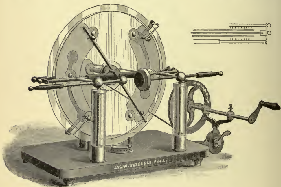
FIG. 11.—Toeppler-Holtz influence machine.
