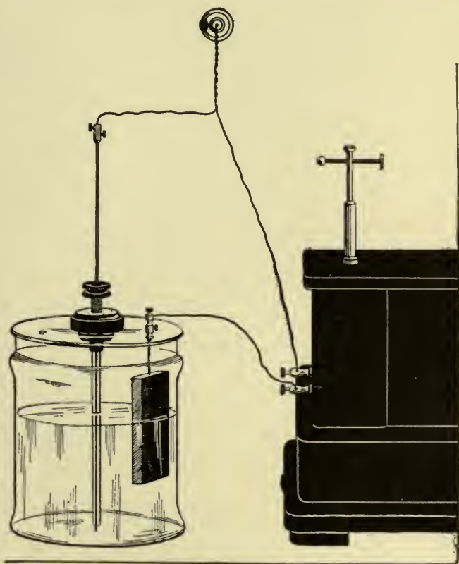
FIG. 76.—Fricklander electrolytic interrupter. The electrolyte is composed of a 10 per cent. solution of magnesium sulphate, and the anode is made of German-silver wire. The operator can control the current for the work in hand by simply turning the thumb-screw. It operates by either the direct or alternating currents.
