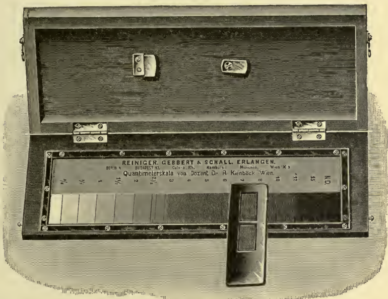
FIG. 221.—Kienböck's quantimeter.
