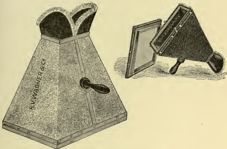
FIG. 104.—Detachable fluoroscope and screen.
